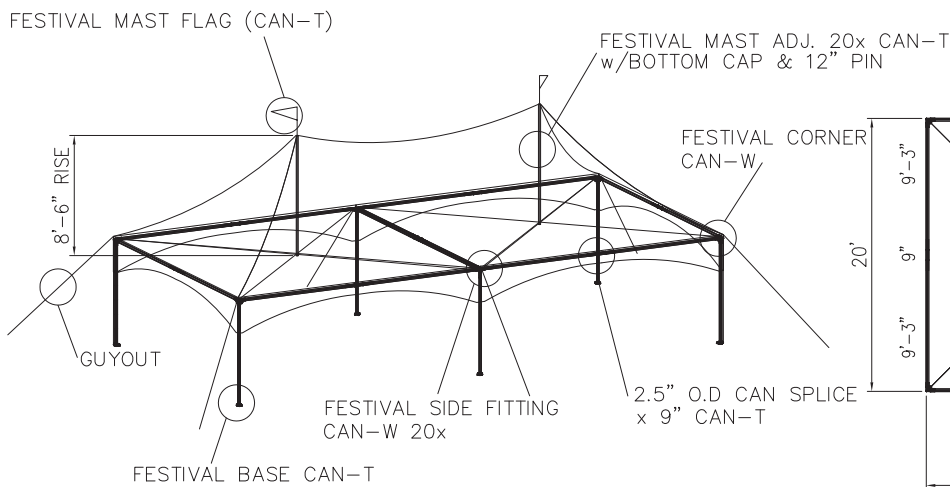
ISOMETRIC VIEW
