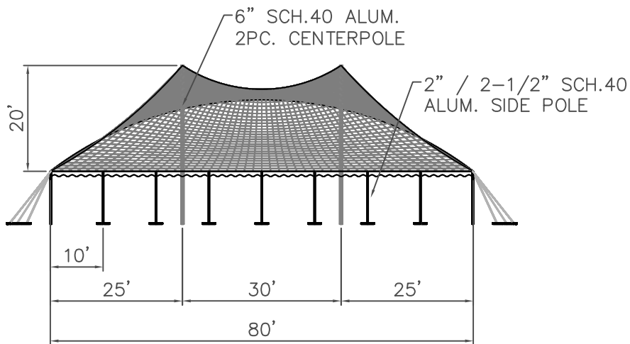
FRONT ELEVATION
