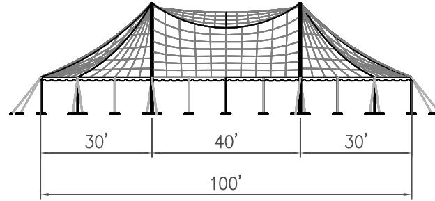
SIDE ELEVATION
