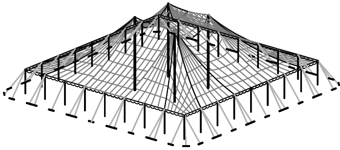
ISOMETRIC ELEVATION
