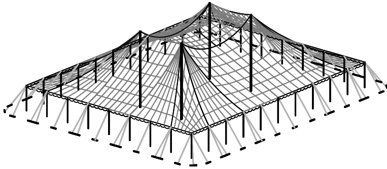
ISOMETRIC ELEVATION
